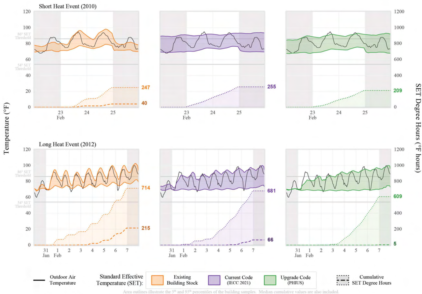
Figure F-18. Existing Single Family: Minneapolis/St. Paul, MN (6A) – Heat Events
