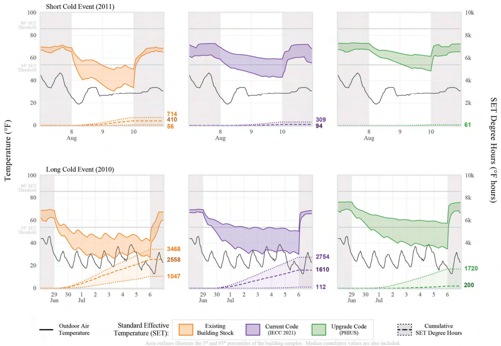
Figure F-8. Existing Single Family: Atlanta, GA (3A) – Cold Events
