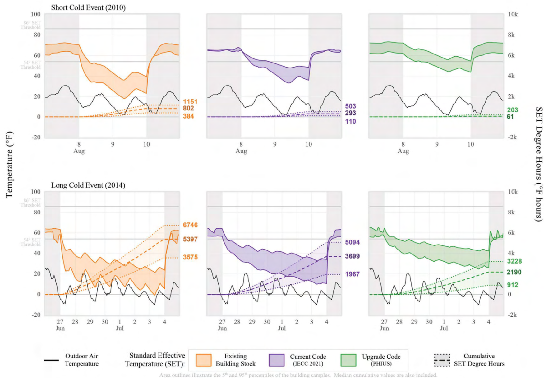
Figure F-12. Existing Single Family: Minneapolis/St. Paul, MN (6A) – Cold Events
