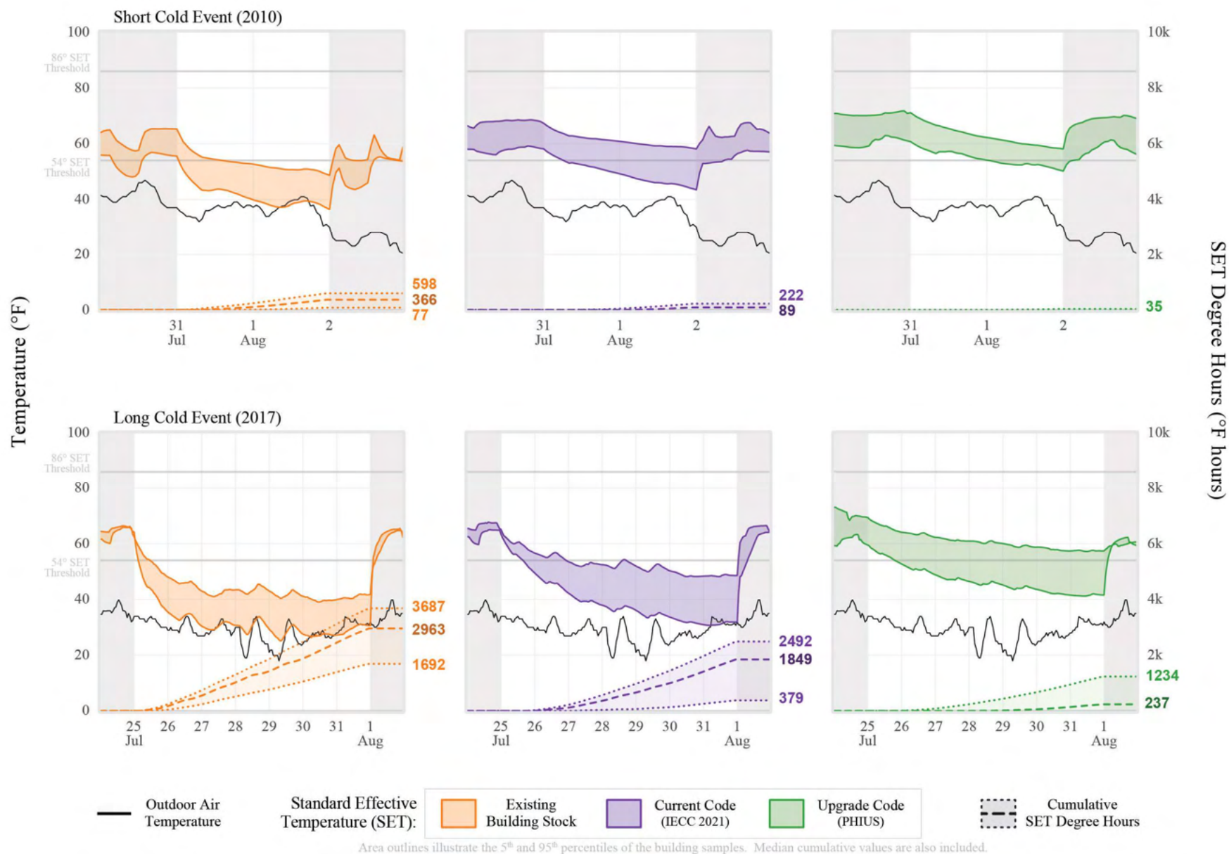
Figure F-10. Existing Single Family: Portland, OR (4C) – Cold Events
