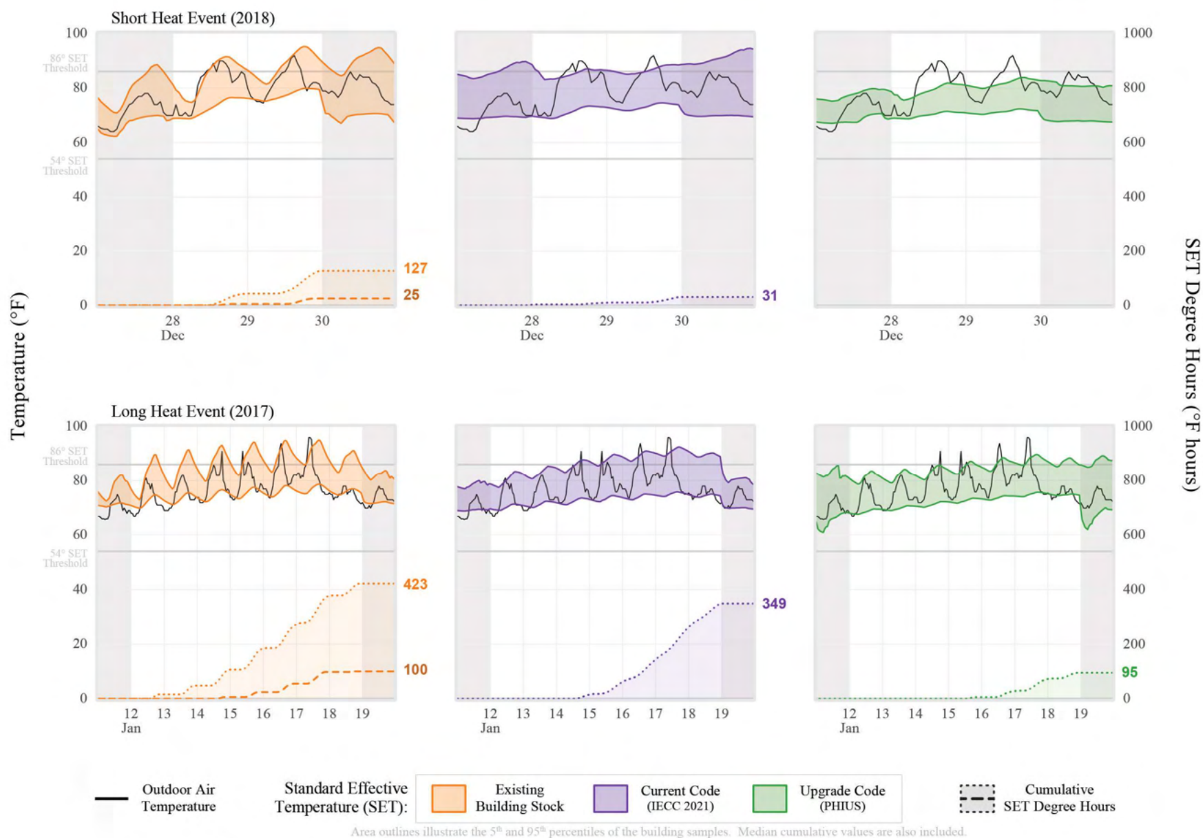
Figure F-15. Existing Single Family: Los Angeles, CA (3B) – Heat Events
