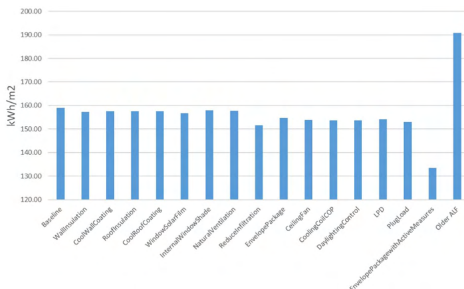
Figure 18. Annual Site EUI of the Baseline and Mitigated Assisted Living Facilities with Passive and Active Measures
